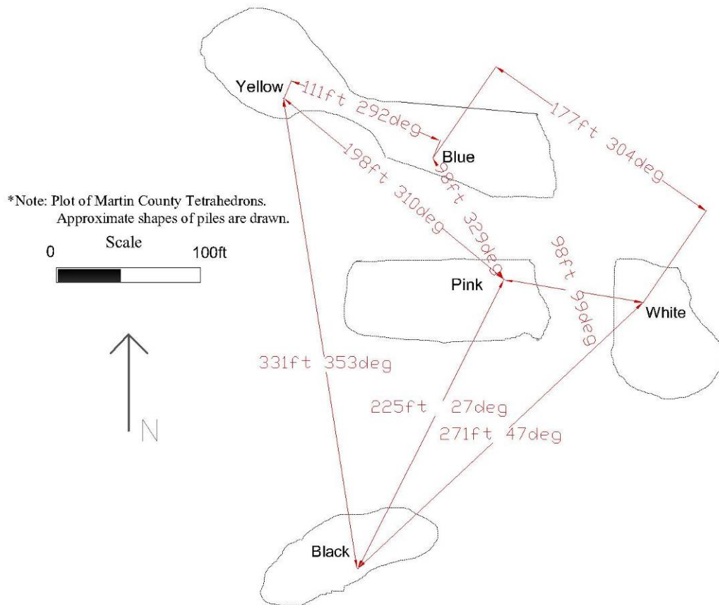
Figure 7. Charts of the Concrete Tetrahedron Patch Reefs
